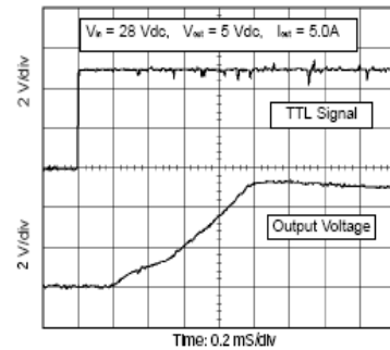
IX. TTL Turn On
