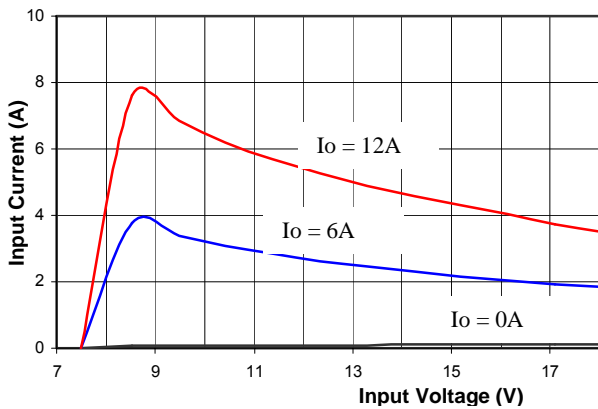
Figure 2. Input Characteristic (5V output)
