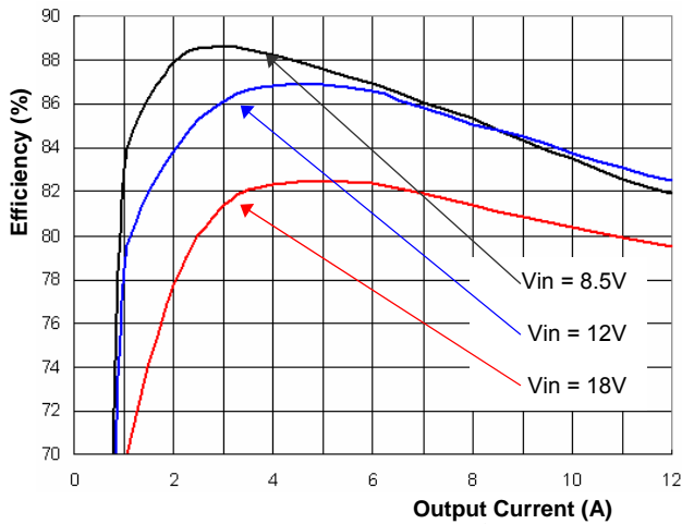
Figure 1(c). Efficiency vs. Load Current (25°C, 1.2V output)
