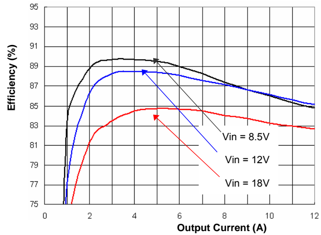
Figure 1(d). Efficiency vs. Load Current (25°C, 1.5V output)
