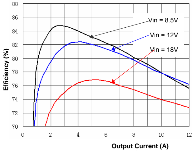
Figure 1(a). Efficiency vs. Load Current (25°C, 0.8V output)
