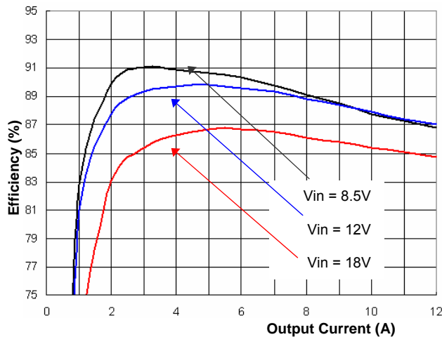
Figure 1(e). Efficiency vs. Load Current (25°C, 1.8V output)
