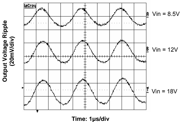
Figure 4. Output Ripple Voltage at 2.5V, 12A Output
