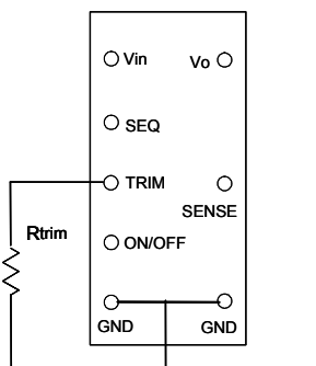
Fig. 15 Circuit to Trim Output Voltage
