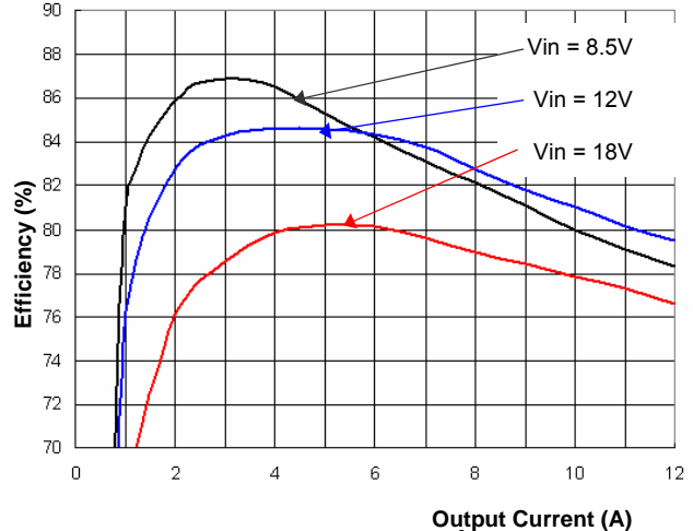
Figure 1(b). Efficiency vs. Load Current (25°C, 1.0V output)
