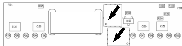
Figure 16. Temperature Monitoring Locations
