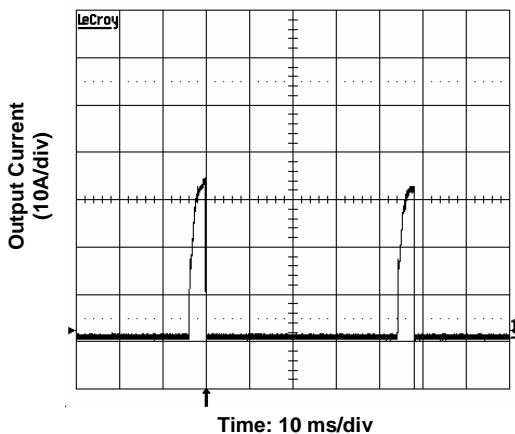
Figure 10. Short circuit current. Vin = 5V.
