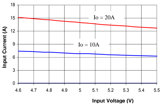
Figure 2. Input Characteristic (output 3.3V)
