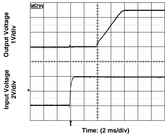
Figure 5. Start-Up from Application of Input Voltage Input voltage 4V, Output current 20A
