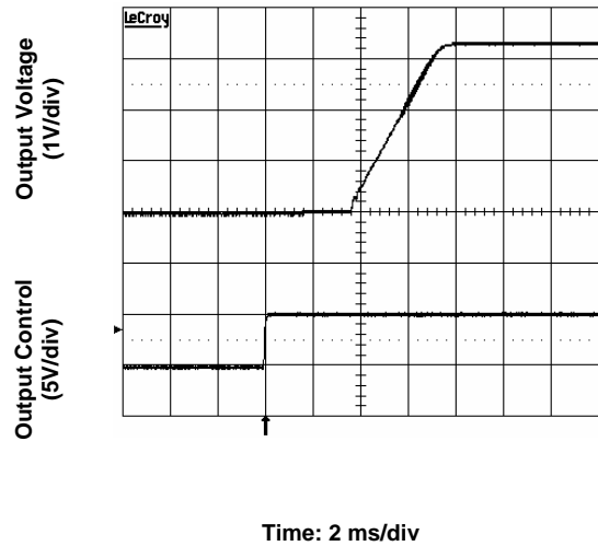
Figure 3. Start-Up from Enable Control Input voltage 5V, Output current 20A
