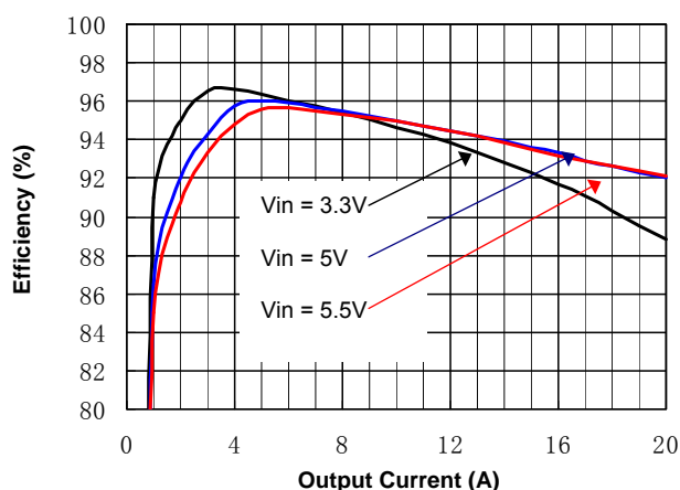
Figure 1(e). Efficiency vs. Load Current (25°C, 1.8V output)
