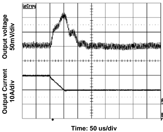
Figure 8. Transient Load Response. Output current 10A (50% full load), Input voltage 5V, Slew rate 0.2A/µs.
