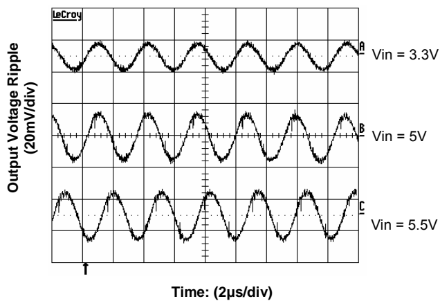
Figure 4. Output Ripple Voltage at 2.5V, 20A Output
