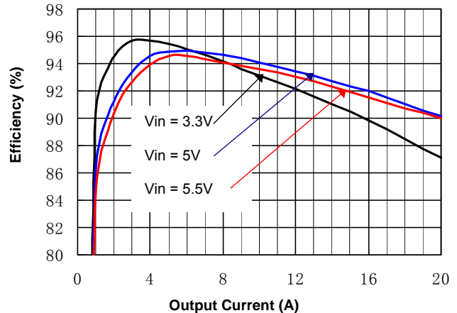
Figure 1(d). Efficiency vs. Load Current (25°C, 1.5V output)
