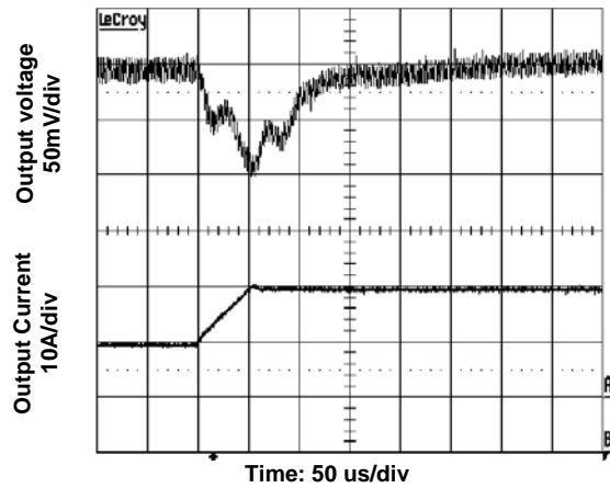
Figure 9. Transient Load Response. Output current 10A (50% full load), Input voltage 5V, Slew rate 0.2A/µs.
