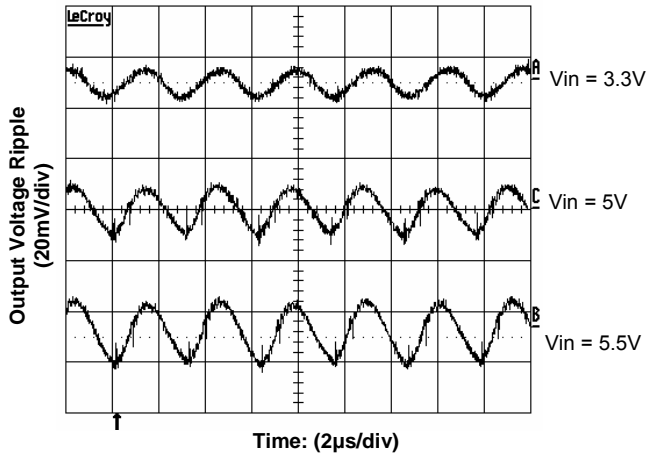
Figure 6. Output Ripple Voltage at 1V, 20A Output
