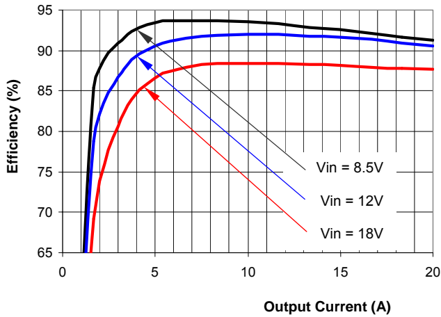
Figure 1(g) Efficiency vs. Load Current (25°C, 3.3V output)
