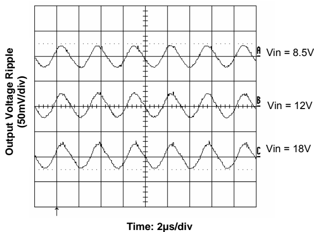
Figure 4 Output Ripple Voltage at 2.5V, 20A Output
