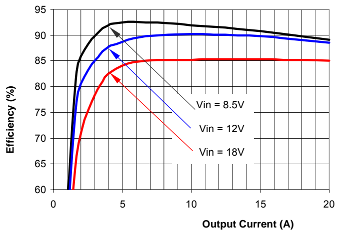
Figure 1(f) Efficiency vs. Load Current (25°C, 2.5V output)
