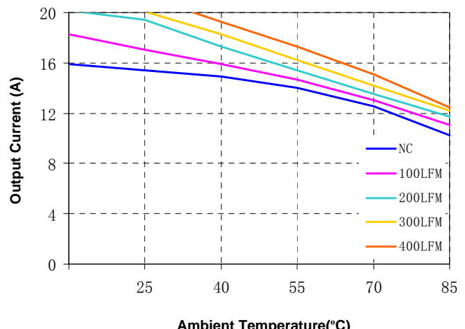
Figure 12(f) Current Derating Curve for 5.0V Output ( Vin = 12V open frame)
