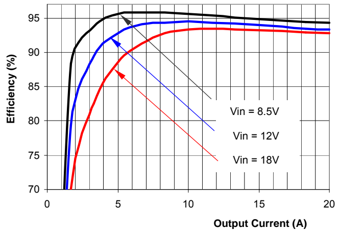
Figure 1(h) Efficiency vs. Load Current (25°C, 5V output)
