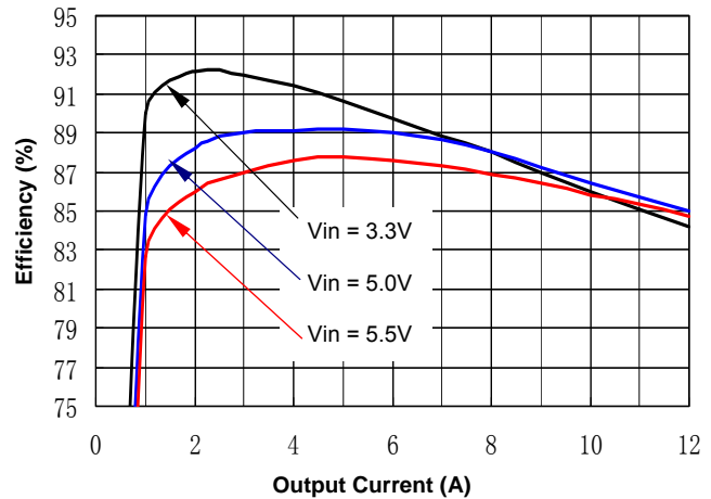
Figure 1(b). Efficiency vs. Load Current (25°C, 1.0V output)
