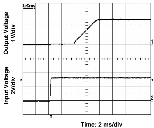
Figure 5. Start-Up from Application of Input Voltage Input voltage 3.3V, Output current 12A
