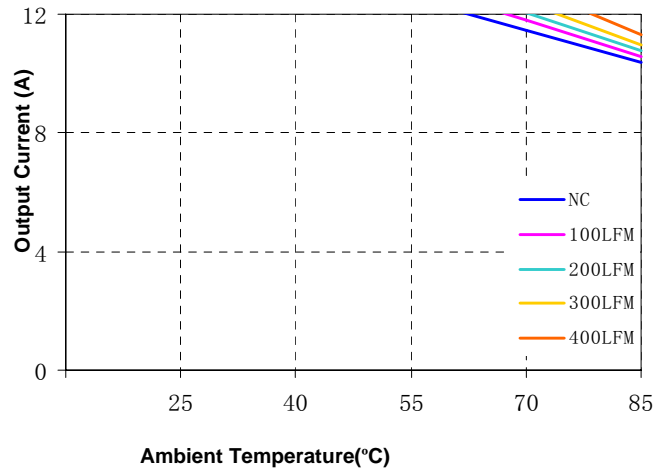
Figure 12(d). Current Derating Curve for 1.8V Output ( Vin = 5V open frame)
