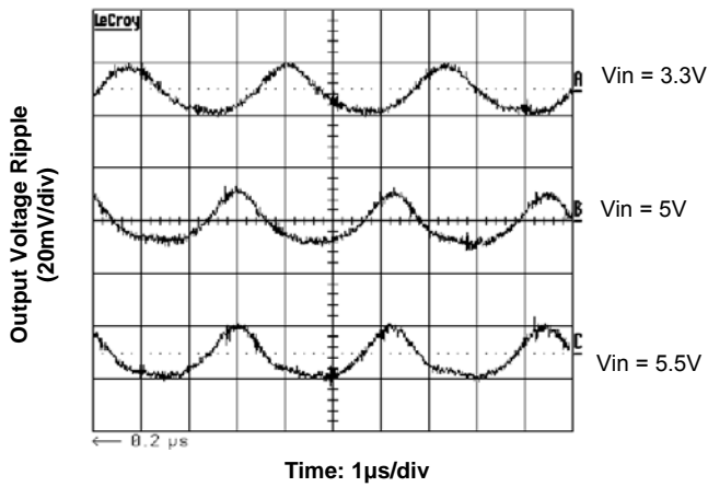
Figure 6. Output Ripple Voltage at 1V, 12A Output
