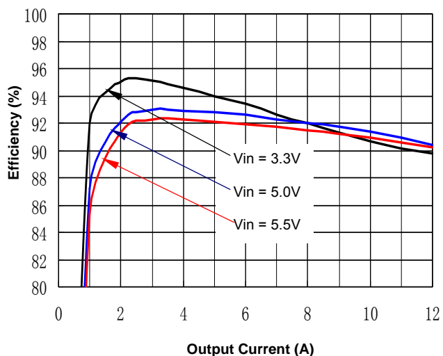
Figure 1(e). efficiency vs. Load Current (25°C, 1.8V output)
