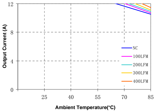
Figure 12(c). Current Derating Curve for 1.5V Output ( Vin = 5V open frame)
