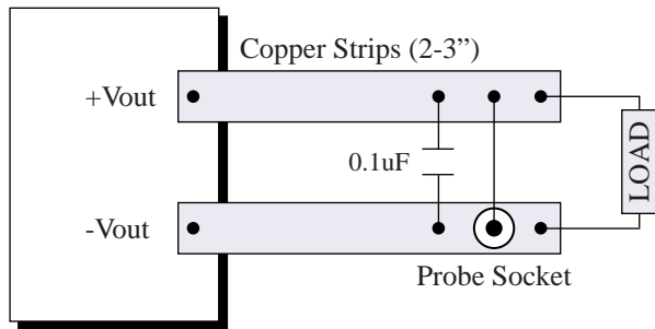
Output Ripple & Noise Measurement
