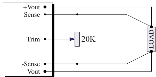
Trim Pot Connection
