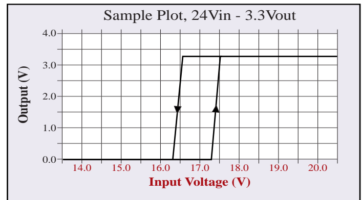
Under-Voltage Lockout
