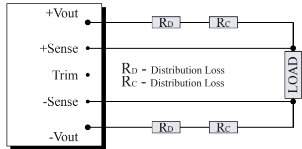
Fig. a Remote Sense Connection
