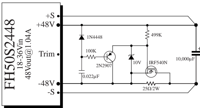
High Capacitive Load
