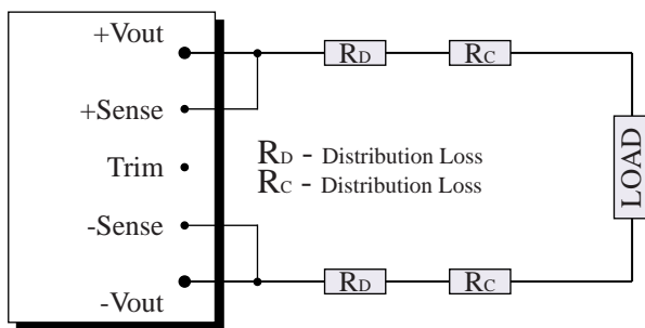
Fig. b Remote Sense is not Used.
