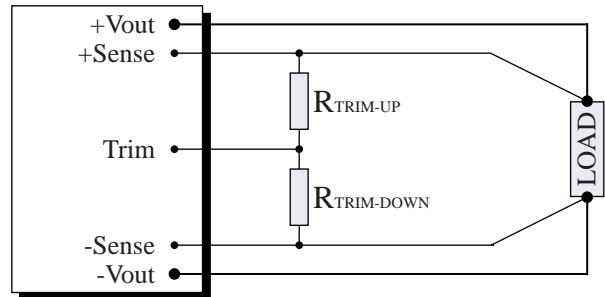
Positive Trim Logic
