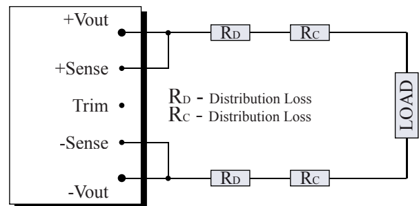
Fig. b Remote Sense is not Used.
