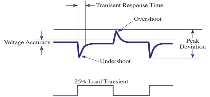
Load Transient
