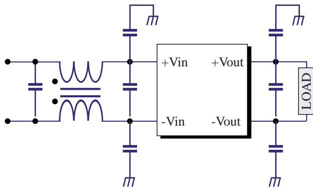
External Common Mode Filter
