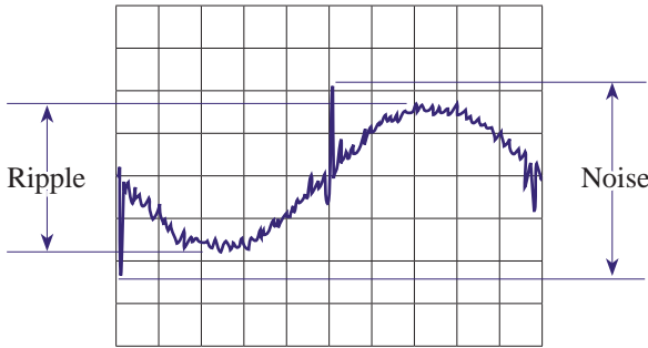
Output Ripple & Noise
