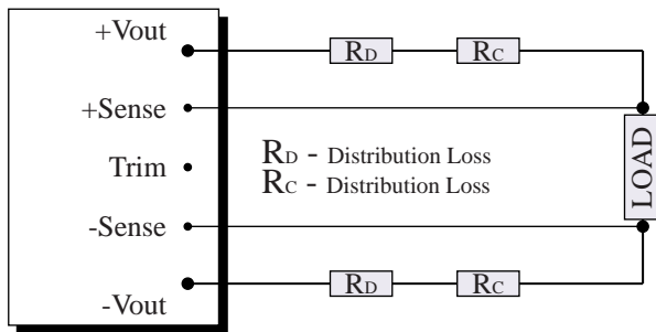
Fig. a Remote Sense Connection
