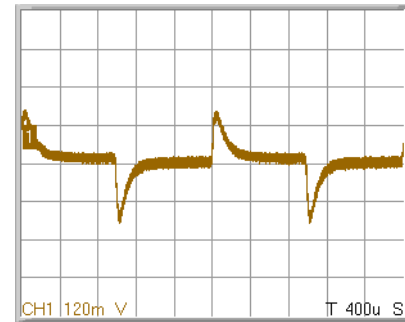
Screen Shot of Load Transient
