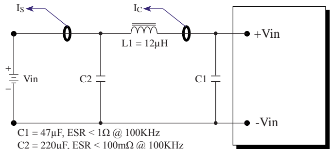
Input Reflected Ripple Current
