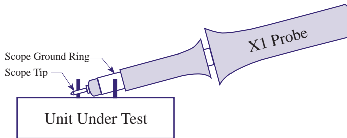
Simplified Ripple & Noise Measurement
